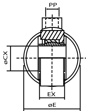
MP5 CAP FIXED SPHERICAL BEARING MOUNTING
