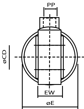
MP3 CAP FIXED EYE MOUNTING
